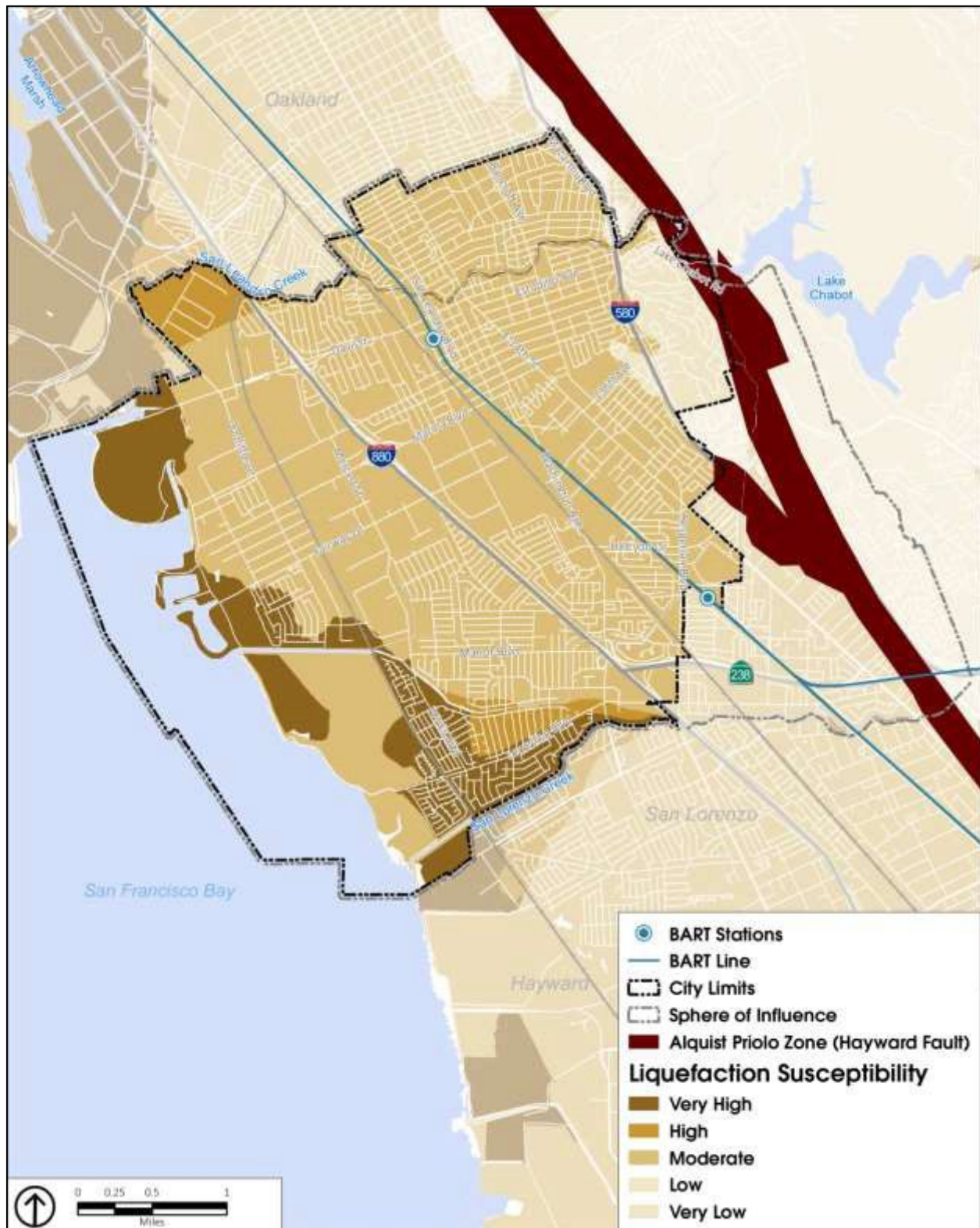
Figure 7-2 Hayward Fault Location and Liquefaction Hazards
