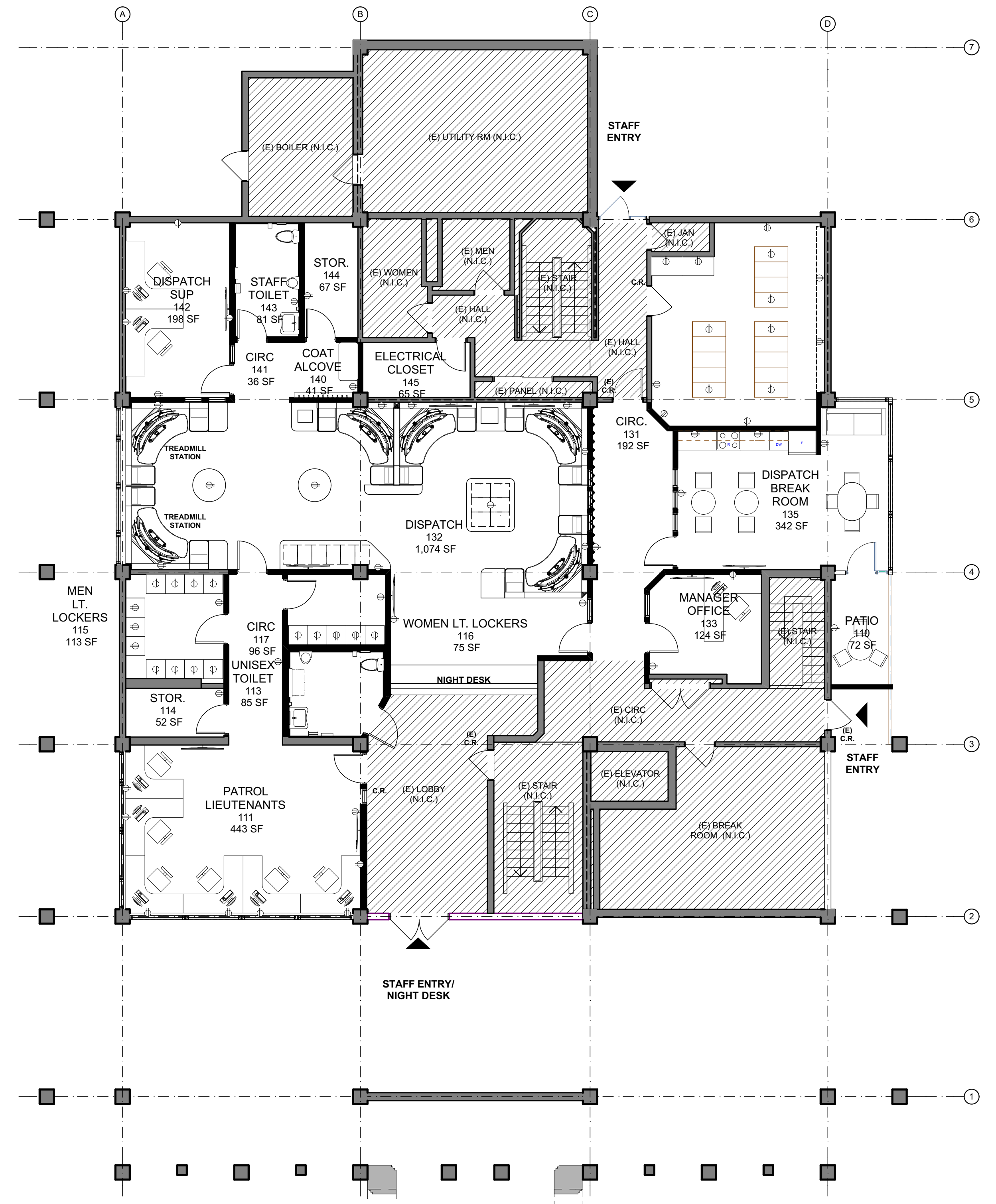
1 FURNISHING REFERENCE PLAN - POLICE BUILDING (BLDG 1) SCALE: 1/8" = 1'-0"
