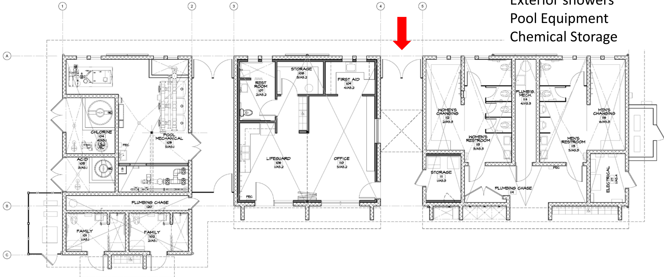
1 FLOOR PLAN 1/4" = 1'-0"
