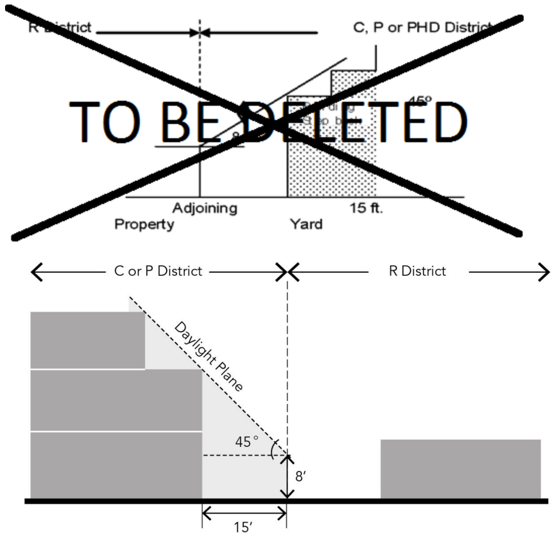
Required Daylight Plane at Adjoining Districts—C, or P or PHD Districts (The diagram is illustrative)
