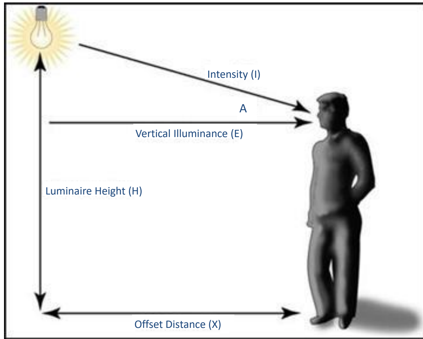
Vertical Illuminance
